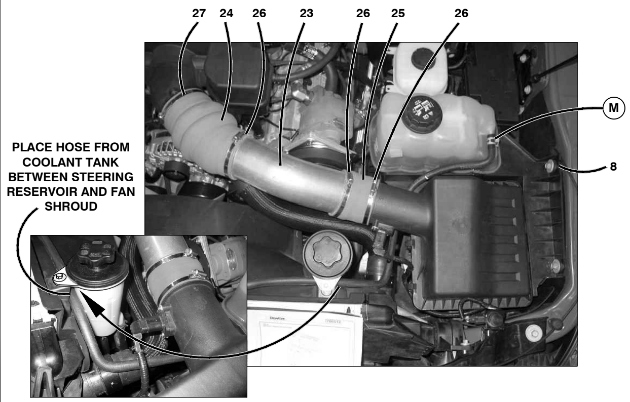
FIG. 4 AIR TUBE REPLACEMENT
