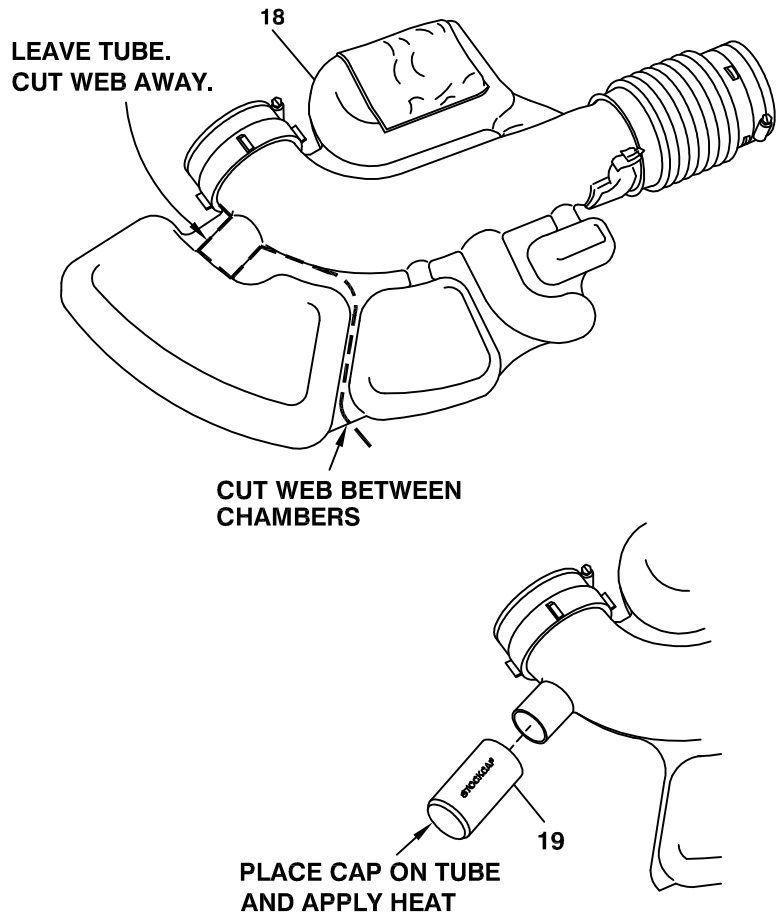
FIG. 3 AIRBOX MODIFICATION
